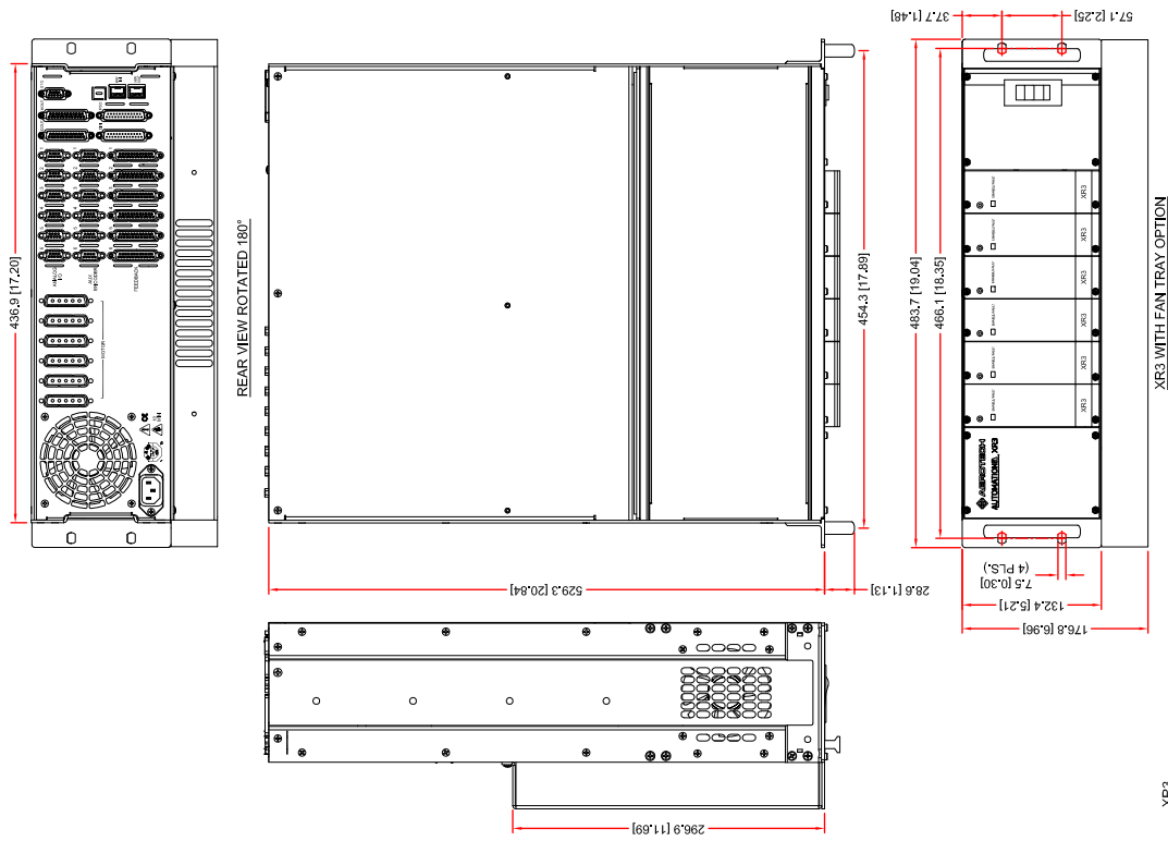
XR3 Dimensions, Rack-Mounted
